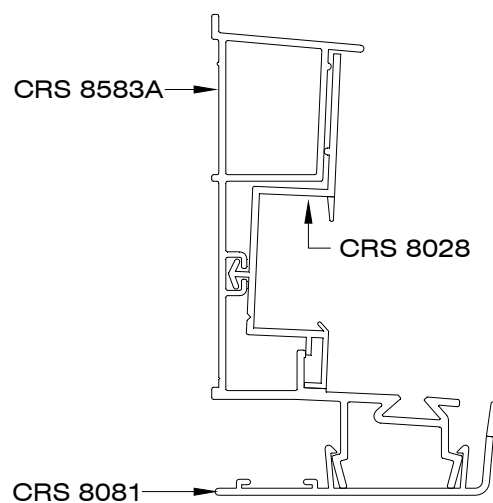
LOW LINE WALL PLATE ASSEMBLY
