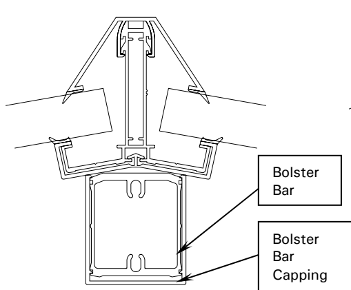
VICTORIAN HIP ASSEMBLY
