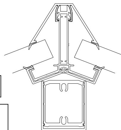
EDWARDIAN HIP ASSEMBLY
