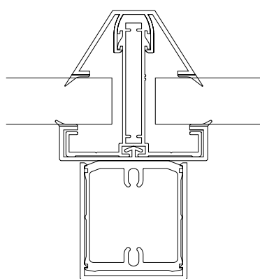
STANDARD RAFTER ASSEMBLY
